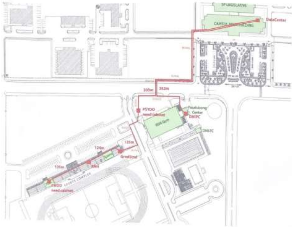
FIBER OPTIC CABLING PROJECT ROUTING MAP Provincial Government of Davao del Norte, Mankilam, Tagum City
